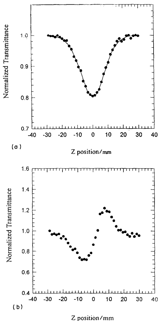
Fig. 17. (a) The NLO absorption of [(PPh_3)_3Cu_2MoOS_3] . (b) The NLO refraction of [(PPh_3)_3Cu_2MoOS_3] .
