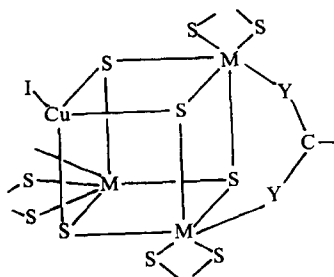
Fig. 13. Tri-Mo(W) clusters.
