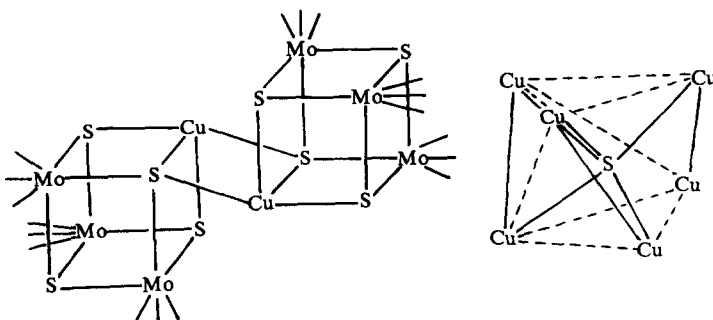
Fig. 14. Hexa-Mo clusters.
