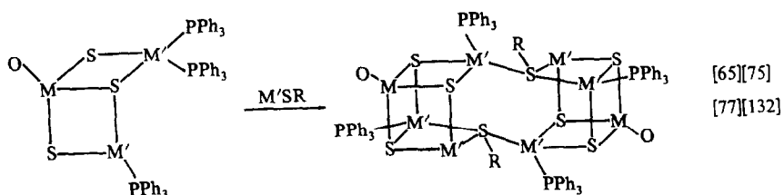
Scheme 4(d). (3+1)+(3+1) reactions.
