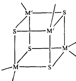
Fig. 8. Tetranuclear clusters.
