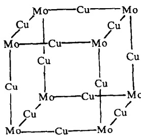
Fig. 15. Octa-Mo(W) clusters.
