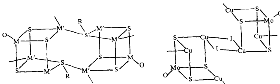
Fig. 12. Octanuclear clusters.
