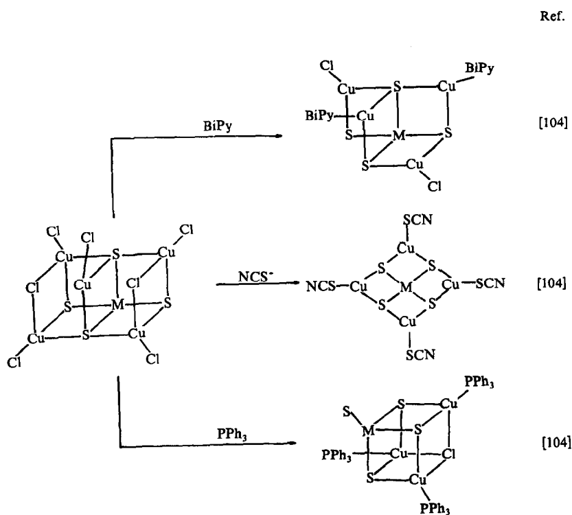
Scheme 5. Decomposition reaction.
