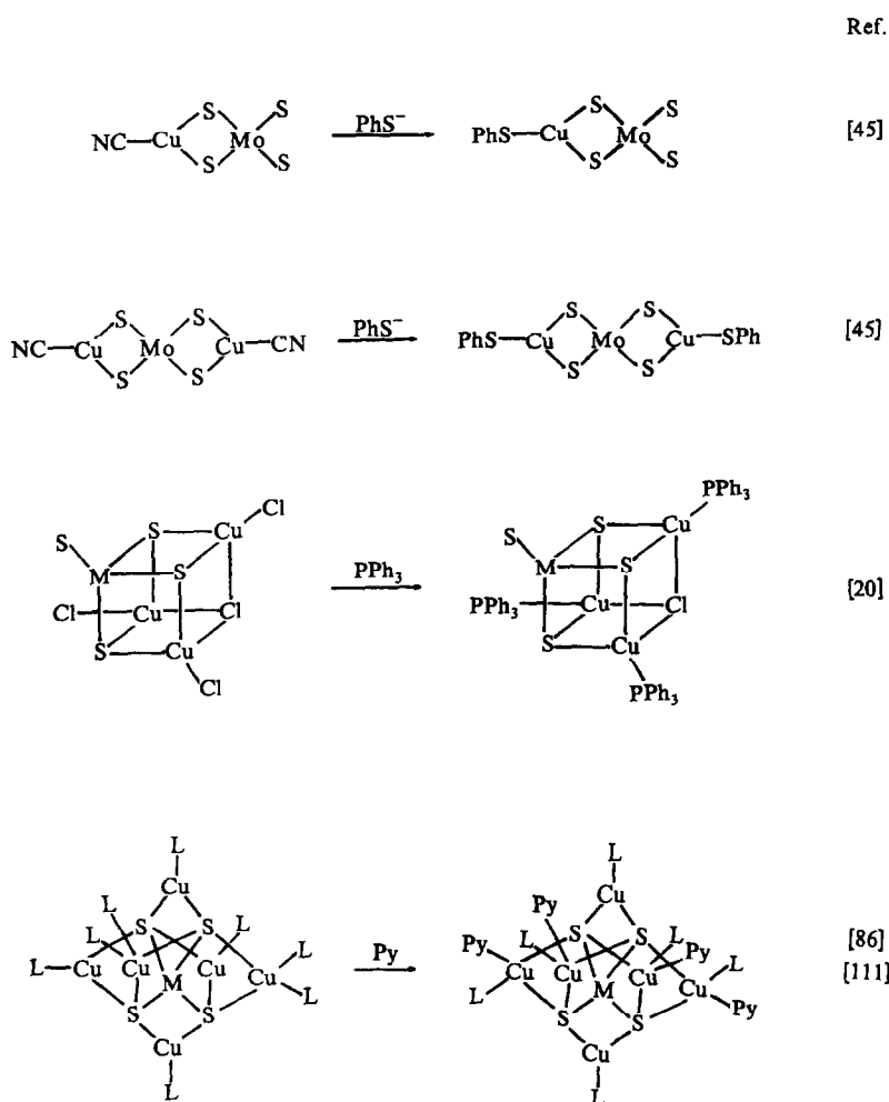
Scheme 2. Substitution reactions of ligands.
