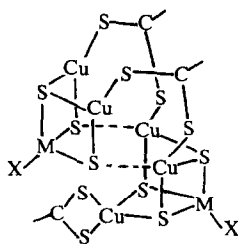
Fig. 11. Heptanuclear clusters.
