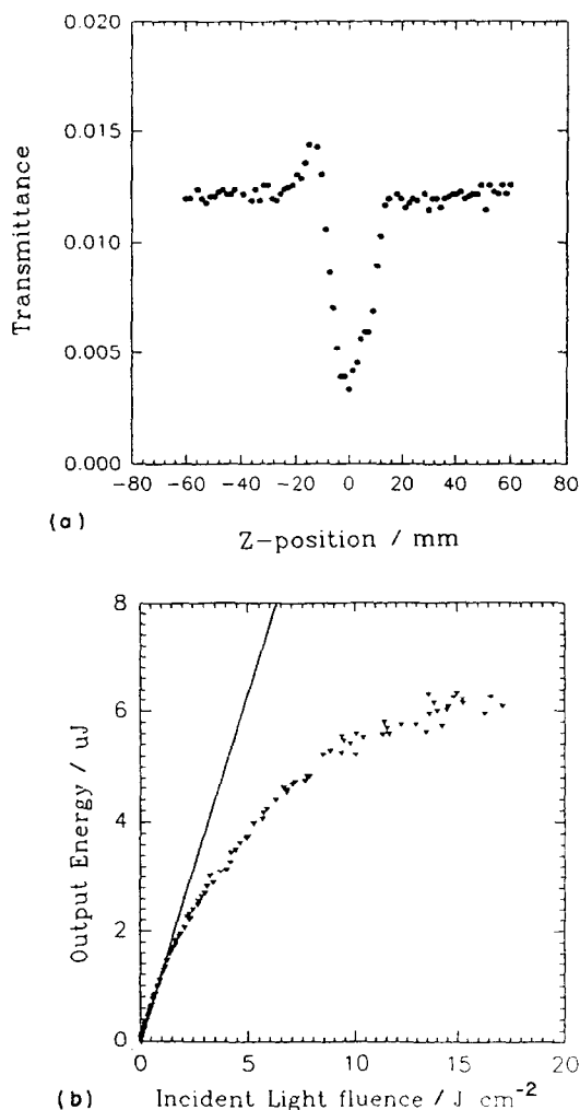
Fig. 20. (a) The self-defocusing ability of [\text{Et}_4\text{N}]_4[\text{Br}_2\text{I}_4\text{Cu}_6\text{Mo}_2\text{O}_2\text{S}_6] . (b) The optical limiting data of [\text{Et}_4\text{N}]_4[\text{Br}_2\text{I}_4\text{Cu}_6\text{Mo}_2\text{O}_2\text{S}_6] .
