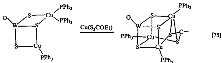
Scheme 4(b). 3 + 1 reactions.
