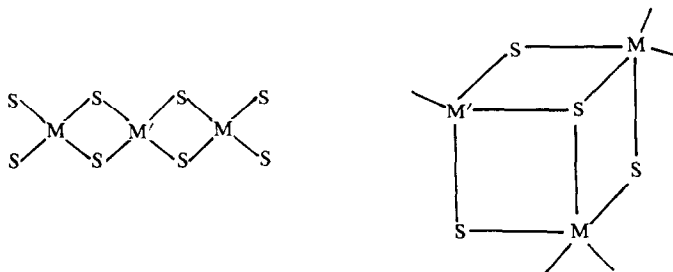
Fig. 7. Trinuclear clusters.
