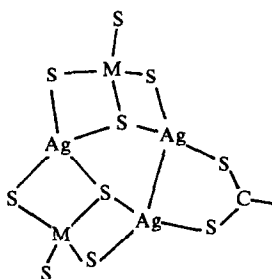
Fig. 9. Pentanuclear clusters.
