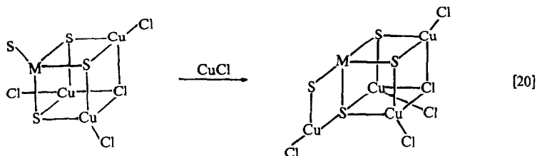
Scheme 4(c). 4 + 1 reactions.
