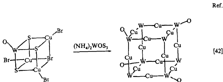
Scheme 4(f). "Co polymerization" reactions.
